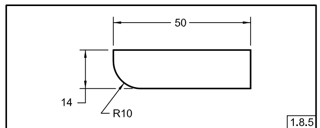
Fig. 1-31 Rounded Corners
