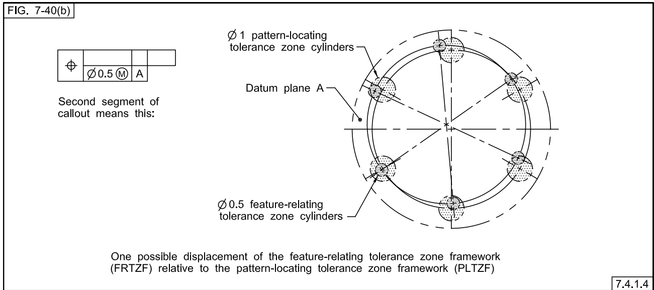
Fig. 7-40 Composite Positional Tolerancing of a Circular Pattern of Features (Cont'd)
