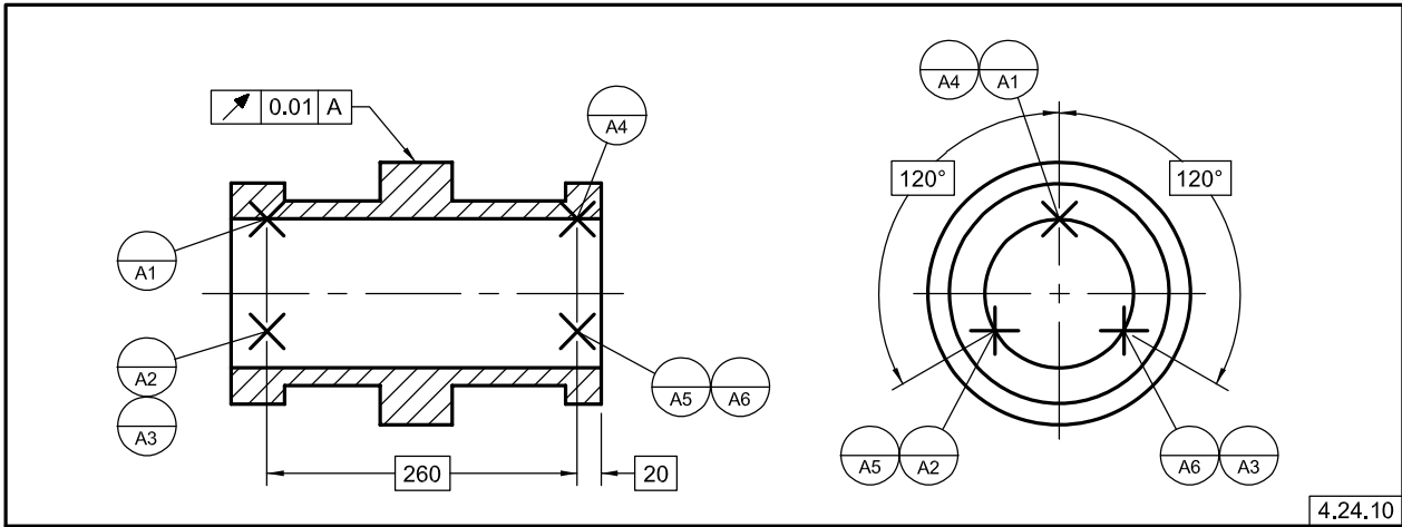
Fig. 4-51 Primary and Secondary Datum Established by Datum Target Lines on Two Cylindrical Features and a Surface
