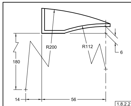
Fig. 1-25 Foreshortened Radii
