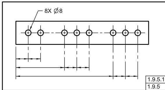
Fig. 1-54 Repetitive Features
