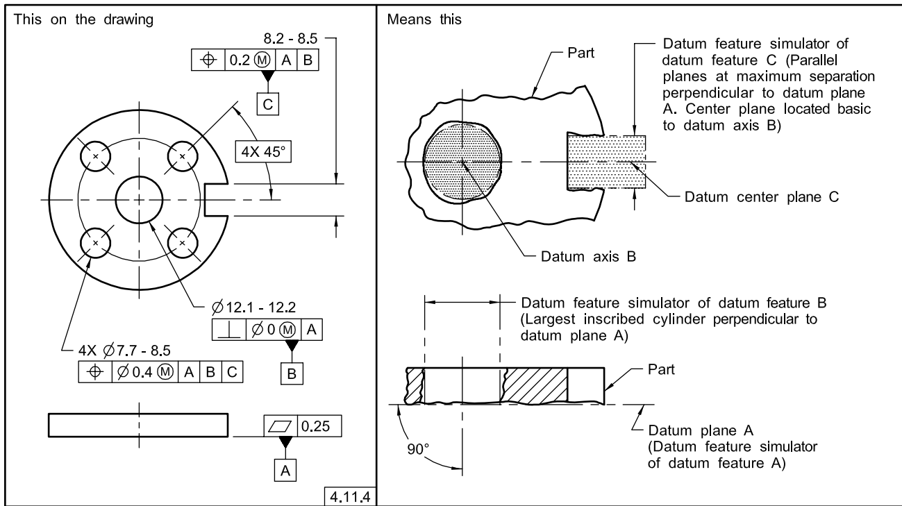
Fig. 4-15 Secondary and Tertiary Datum Features — RMB
